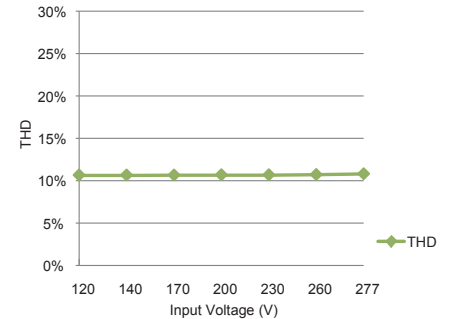
THD vs Input Voltage
